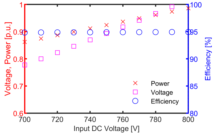
Fig. 7. Output voltage, power, and DC-DC efficiency from a parametric sweep of input DC voltage between 700 and 800V. Altering the DC input voltage offers the most power reduction with limited impact on efficiency.
