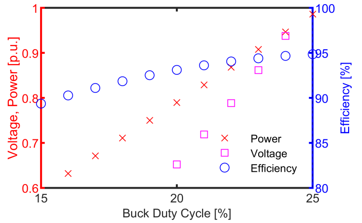
Fig. 8. Output voltage, power, and DC-DC efficiency from a parametric sweep of buck converter duty cycle between 15 and 25%. Buck converter modification can significantly reduce power but has a large impact on voltage.
