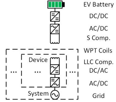
Fig. 1. A prototype transmitter and receiver coil pair for wireless charging testing and a diagram of an example wireless power transfer system for charging electric vehicles with power-systems level control and power electronics control to compensate for variability. Models employed in this study are based on previously published prototypes from ORNL experimentally validated at 85kHz, 120kW operation and simulated up to 200kW [1].
