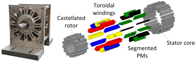
Fig. 1. Prototype and exploded view of existing high power density motor using a PM free castellated inner rotor and a modular stator with concentrated toroidal coils and tangentially magnetized PMs.
