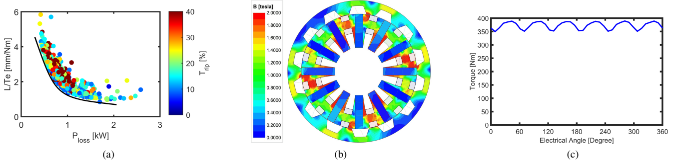
Fig. 8. (a) Optimization results projected for torque - total loss plane showing torque ripple variation , (b) cross-sectional view of the selected "best" design OR-PM D1 with a plot of the flux density and lines, and (c) torque waveform of selected "best" design OR-PM D1.
