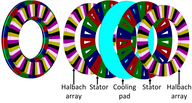
Fig. 3. Assembled and exploded view of the coreless axial flux PM (CAFPM) synchronous motor unit. The twin Halbach array PM rotors contribute a high airgap flux density, and the integrated cooling pad enables high current density.
