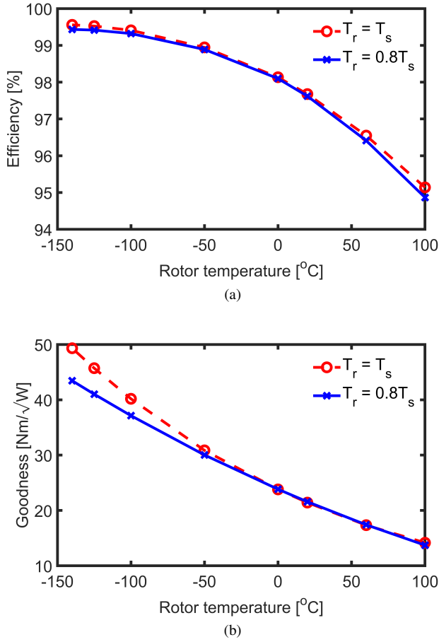
Figure 3. Efficiency (a) and Goodness (b) under two scenarios: (1) equal rotor and stator temperatures, and (2) rotor temperature at 80% of the stator temperature, evaluated across a range from high to cryogenic temperatures.
