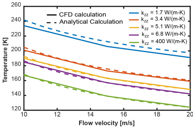
Figure 6. Average stator coil temperature for different thermal conductivities and varying flow velocity.
