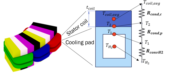
Figure 4. Geometry of the AFPM motor and its corresponding simplified thermal circuit.
