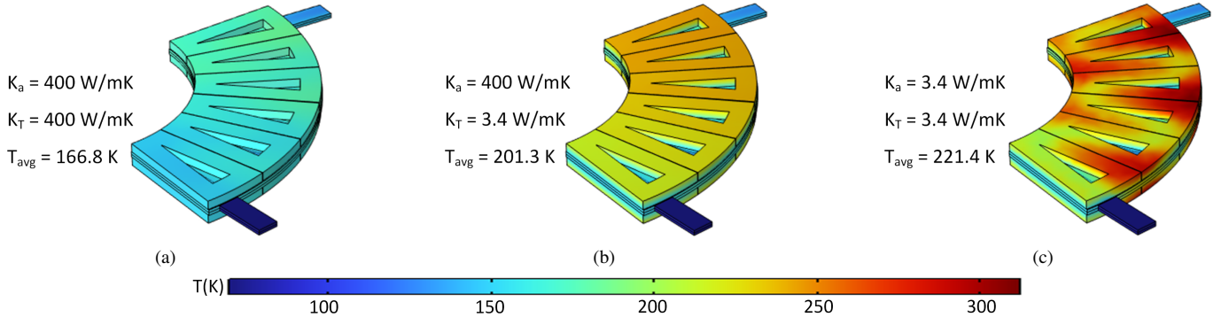
Figure 5. Simulation results for non-isotropic thermal conductivity when (a) k_T = k_A = 400 W/mK, (b) k_T = 3.4 W/mK and k_A = 400 W/mK, and (c) k_T = k_A = 3.4 W/mK.
