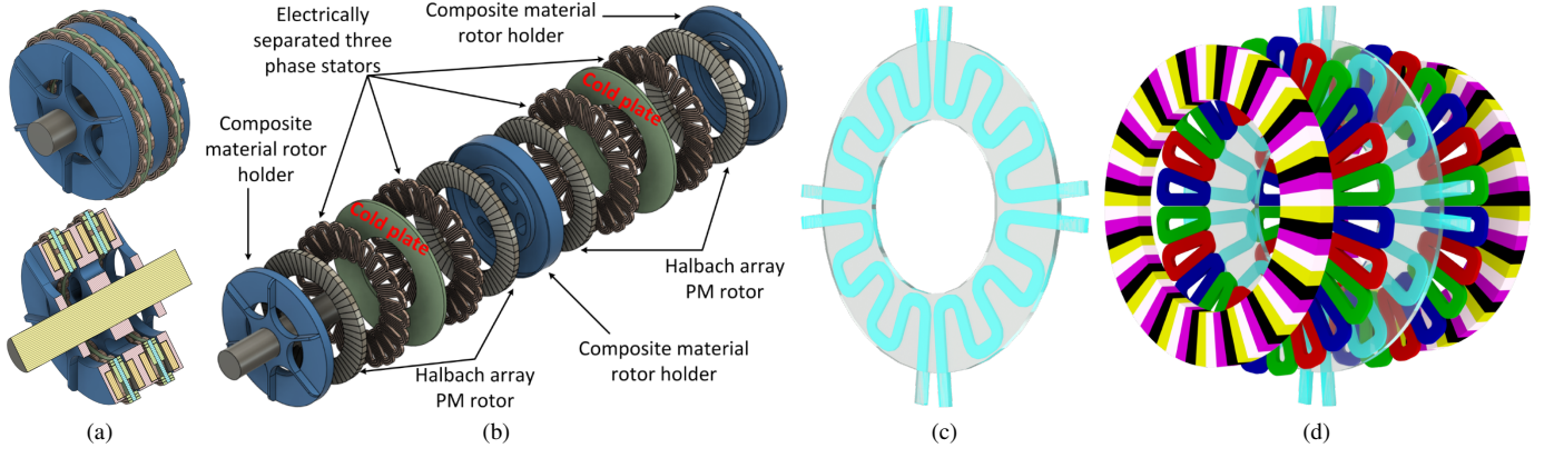
Figure 1. Proposed coreless AFPM machine with an integrated cryogenically cooled thermal management system, illustrating (a) compact and sectional views of the double-stage design, (b) the exploded view of the full assembly, (c) the topology of the cold plate positioned between the two stators in each module, and (d) the exploded view of a single stage.
