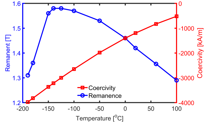
Figure 2. Remanence and coercivity curves of NdFeB 50BH at various temperatures.
