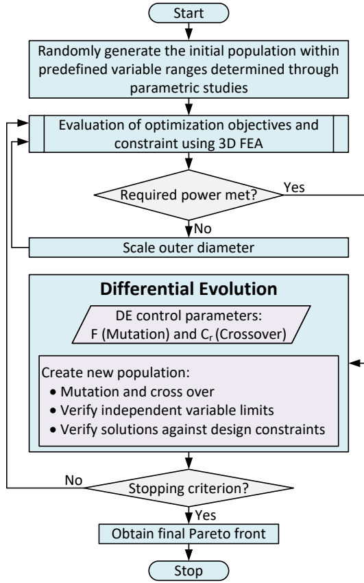
Fig. 6. The proposed optimization algorithm based on the combination of the differential evolution method and 3D FEA.
