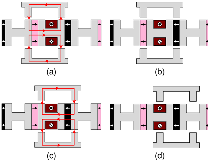
Fig. 3. Operating principle of the proposed AFPMG-RR from a generator-oriented perspective, illustrating positions where flux linkage in the coil is at (a) maximum, (b) zero, (c) minimum, and (d) zero.
