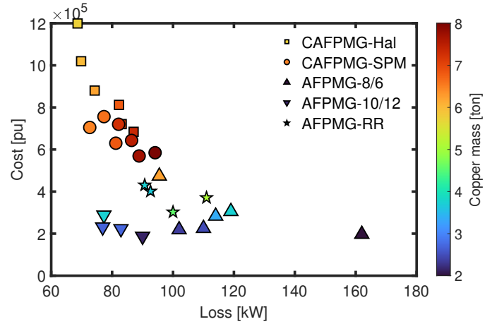
Fig. 10. Pareto front design candidates for all five generator concepts, plotted based on a consistent per-unit cost system.
