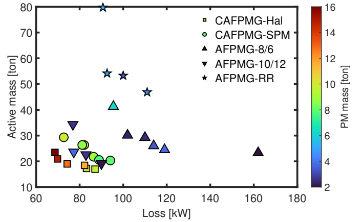
Fig. 7. Pareto front design candidates for all five generator concepts, with all designs rating 3 MW of power at 15 rpm.
