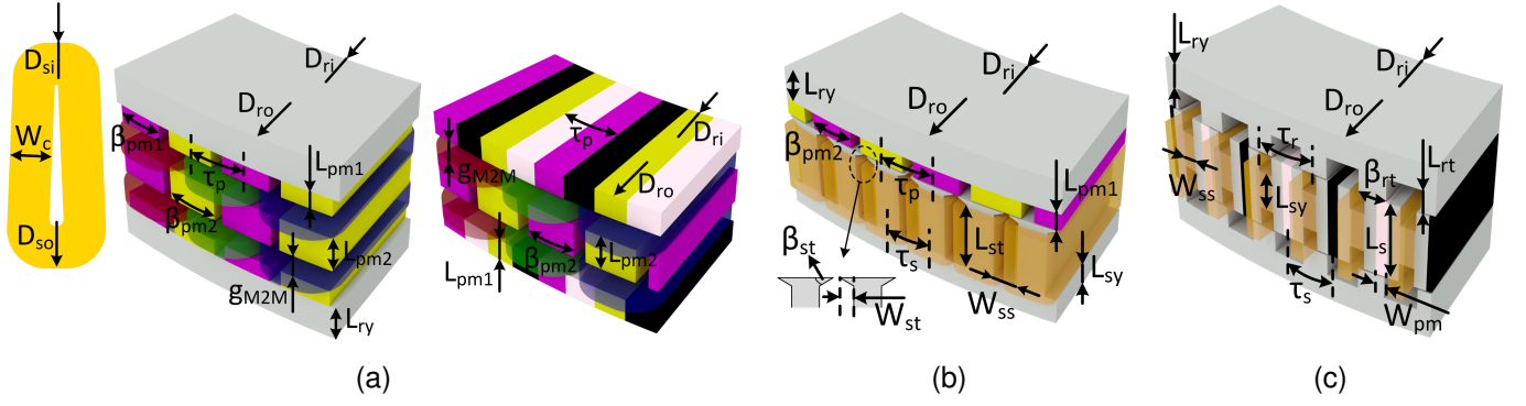
Fig. 5. Geometric design variables applied in the parametric model for the multi-objective optimization, shown for (a) CAFPMGs with surface-mounted PM and Halbach array rotors, (b) conventional AFPMG, and (c) AFPMG-RR configurations.
