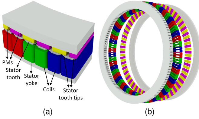
Fig. 2. Conventional single-sided AFPM generator with a 10/12 pole-to-slot ratio (AFPMG-10/12), showing (a) labeled active electromagnetic components and (b) an exploded view of an example design.
