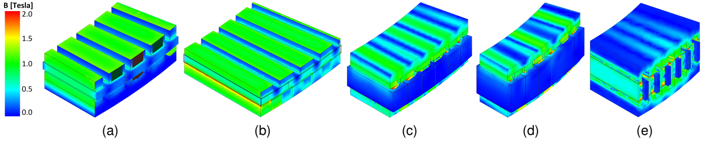
Fig. 8. Flux density distributions for the optimal designs of (a) the half-axial model of CAFPMG-SPM, (b) the half-axial model of CAFPMG-Hal, (c) AFPMG-10/12, (d) AFPMG-8/6, and (e) AFPMG-RR.
