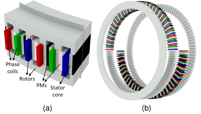
Fig. 4. Axial flux generator concept with combined PM and AC excitation on the stator and double-sided reluctance rotors (AFPMG-RR), showing (a) labeled active components and (b) an exploded view of an example design.
