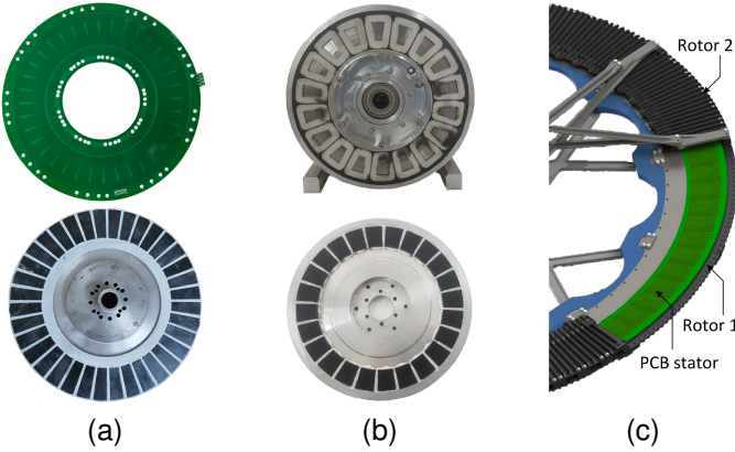
Fig. 9. Coreless stator AFPM machine prototype with surface-mounted PM rotor (a), the conventional single-sided AFPM machine prototype (b), and the coreless AFPM generator with PCB stator designed by Boulder Wind Power, used for the verification of the developed FEA models and calculations.
