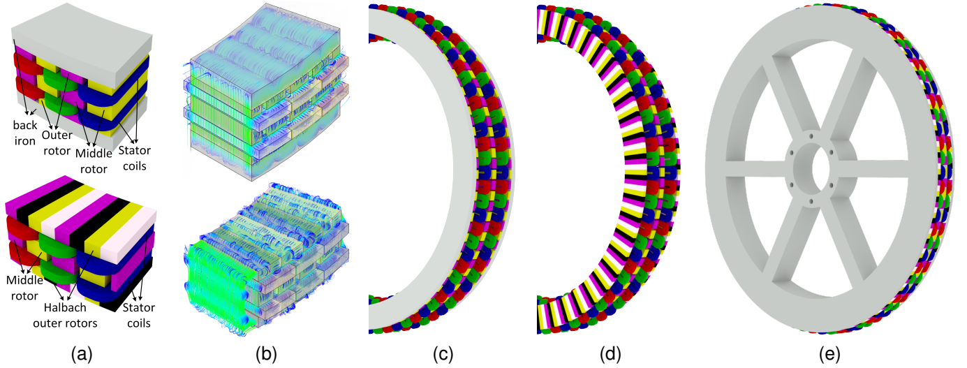
Fig. 1. Coreless stator axial flux permanent magnet generator (CAFPMG) concepts with surface-mounted and Halbach array PM rotors proposed for direct-drive wind turbines. (a) highlights the labeled active components; (b) shows the flux density distribution, with the rotor back iron removed in the Halbach array PM variant; (c) and (d) present slightly exploded views of the two configurations in an example design; and (e) illustrates a simplified mechanical structure for the Halbach array rotor variant, incorporating composite materials.
