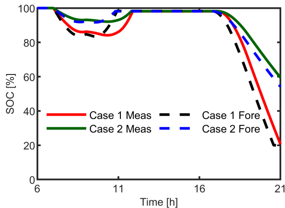
FIGURE 16. Battery SOC over both Scenario 1 and Scenario 2. The batteries discharge in the early morning and recharge during times of excess PV generation.
