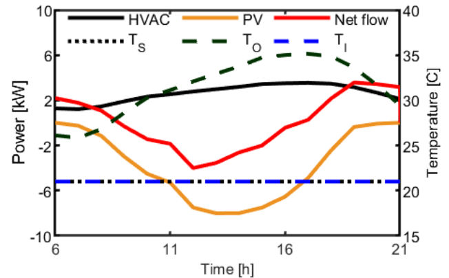
FIGURE 15. Representative plots for SHINES House #1 on July 12, 2020. The house is transformed into a NZE house via scaling with a factor of 2.353 for the annual PV generation and total energy use.
