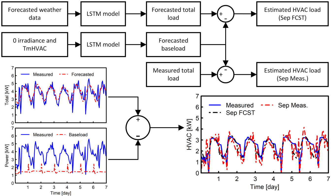
FIGURE 7. Schematic diagram of the mathematical algorithm for the novel HVAC separation method for individual residences. Total load and baseload forecasts are illustrated in the two smaller graphs and an example week from July 16 to July 22, 2020 of the HVAC separation from the total forecasts (Sep FCST) and the total measured data (Sep Meas.) is shown in the larger plot. The separated HVAC load for the summer of 2020 is satisfactory but not as accurate as the forecasts from HVAC measured data shown in Section V.
