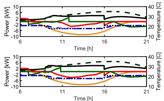
FIGURE 18. Scenario 2: Both the measured PV (top) and forecasted PV (bottom) based HVAC controls result in 0 kWh purchased from the grid during the day with a 27 kWh battery. The only demand-related cost to the user in a 24 hour period is for recharging the battery at night when ToU rates are cheaper.
