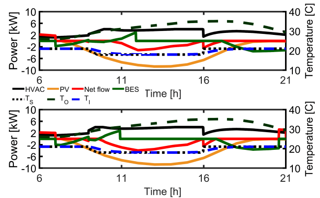
FIGURE 17. Scenario 1: day-ahead load shifting schedule for HVAC based on PV generation (measured top, forecasted bottom) with 13.5 kWh of battery capacity. The forecast of PV ends slightly earlier than the measured data thus causing the positive net power flow at night.
