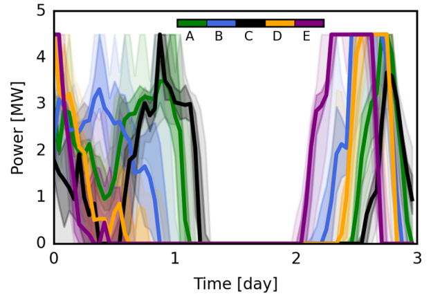
Fig. 8. Time-series wind power for each of the example clusters with darker transparent shading added for the middle 50% and lighter shading for the enter range of the clustered 50km \times y squares. Stopping and starting of wind power intentionally selected to show distinctive behavior between zones.
