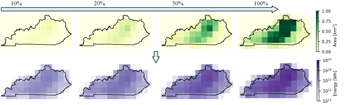
Fig. 4. Designated land area, a_d(x, y) , across the example state excludes a buffer of 200m around roads and urban city areas and was scaled in percentage from lower impact to higher impact. The corresponding SunPower SPR-X21-470 example solar PV annual energy in 2020 for each percentage, visualized on a logarithmic scale, suggests a high potential energy region in central KY. Spacing between rows for a 50% packing factor shows the high end of the range of energy provided in Table I.
