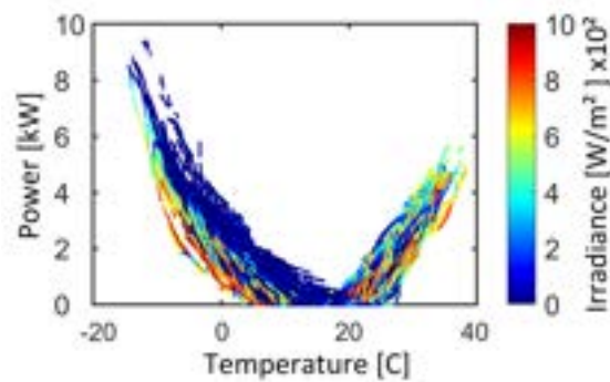
Fig. 3. Example HVAC “V-curve” and physical relationship between weather parameters and power captured by the ML model. In principle, the ML model may be applied with weather at different locations and employ the approximately linear trends to estimate the power demand.
