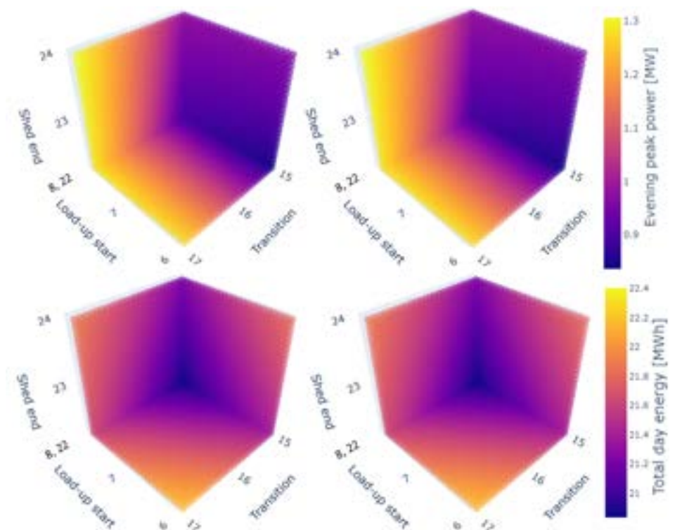
Fig. 9. Response surfaces for the CC (left) and FF (right) DOEs serve as a sanity check for the optimization by indicating the relationship between the independent variables and the optimization objectives. In application of the optimization on different distribution circuits, the CC and FF may be run quickly first to estimate the benefit of the VPP controls.
