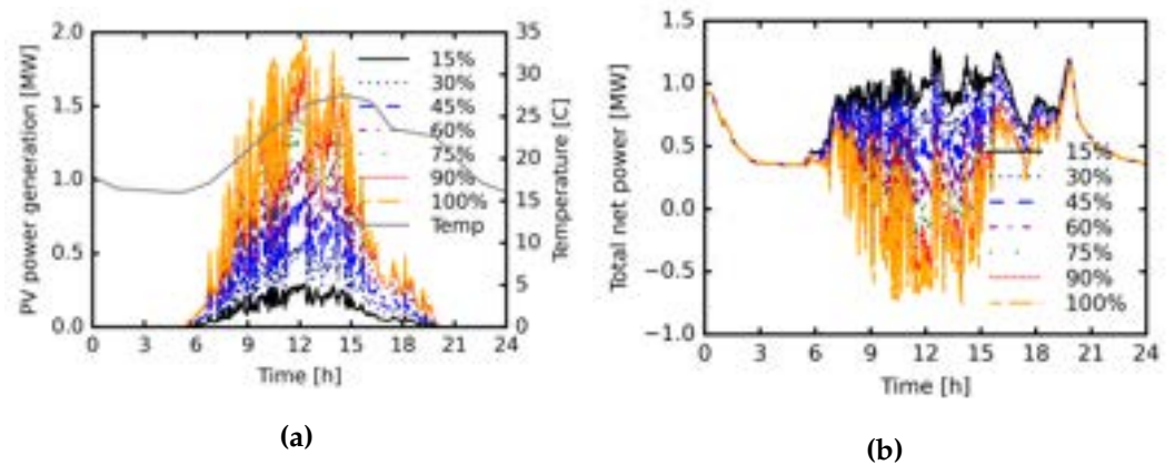
Fig. 6. Results for the (a) distribution system total solar PV power generation and (b) total net power for the simulated 15% and estimated solar PV penetration cases of up to 100%. The variability in solar PV power generation is caused by variability in irradiance.
