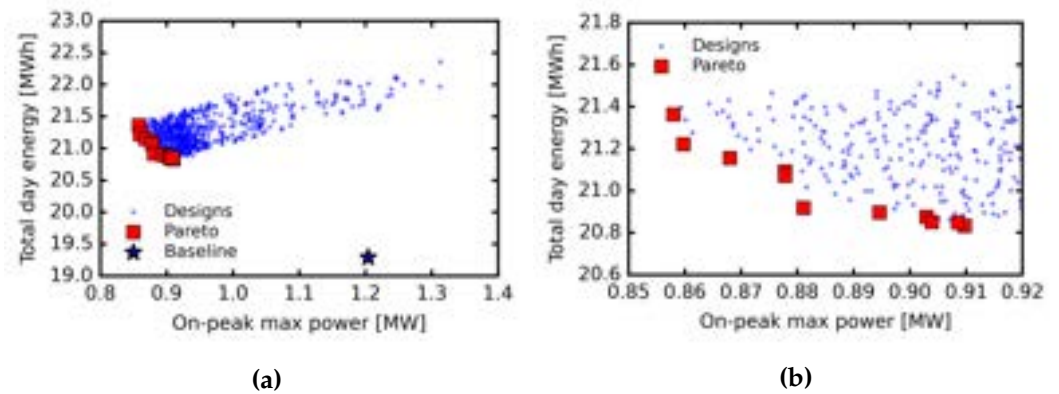
Fig. 10. Resulting (a) objective evaluations and (b) a cropped view of all cases simulated during the NSGA-III optimization with respect to the baseline case and with the Pareto front of the eleven (11) best cases indicated.
