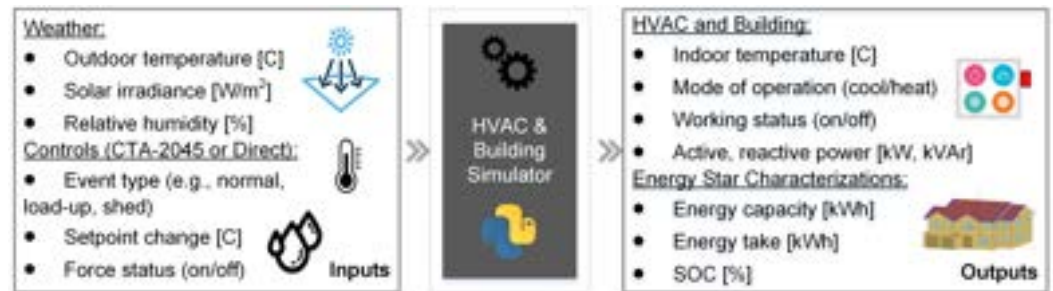
Fig. 2. Visual depiction of the time-dependent HVAC and building simulator. Explicit CTA-2045 commands are issued, and Energy Star GES performance metrics, such as energy take, equivalent SOC, and electric energy capacity, may be estimated through the building simulator.
