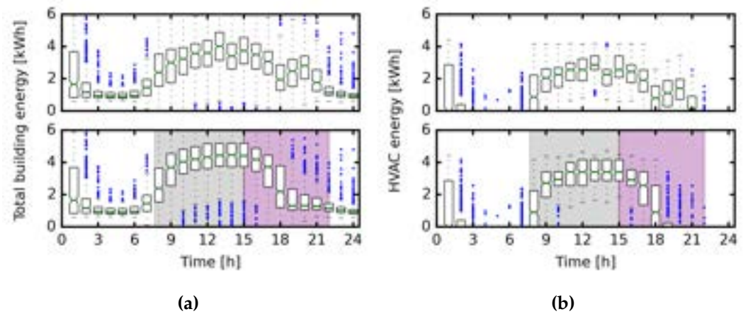
Fig. 12. Results for individual building (a) total energy use and (b) HVAC energy use only of the baseline and P6 cases.
