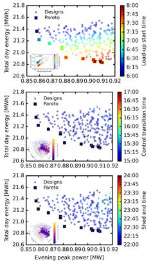
Fig. 11. Relationships between the two (2) objectives and the three (3) independent variables of control times for all simulated cases during the optimization.
