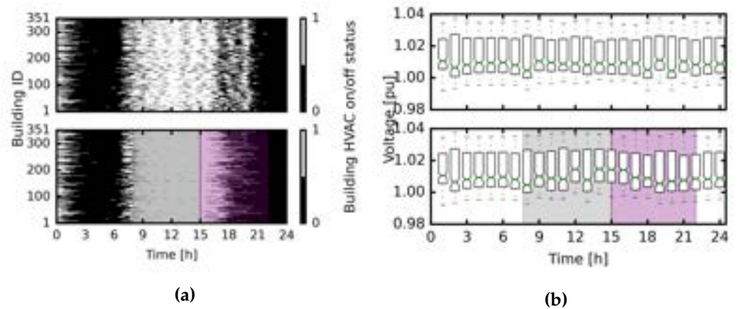
Fig. 7. Simulation results for (a) individual on/off statuses for HVACs to show control phasing in the baseline case (top) and in case P6 (bottom) as well as (b) hourly average bus voltages for both the baseline and P6 cases. The “load-up” and “shed” event windows are shaded in light gray and purple, respectively. This format is replicated in following figures.
