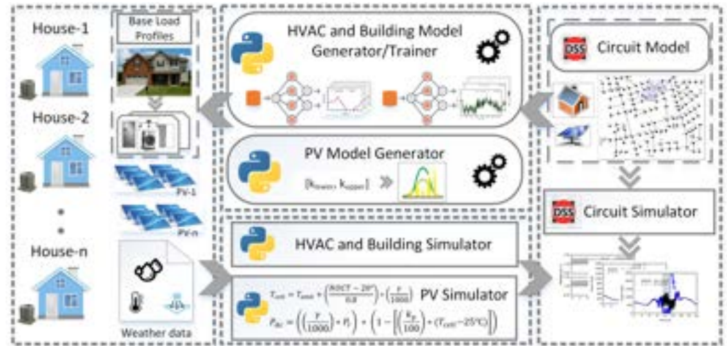
Fig. 1. Visual depiction of the novel co-simulation testbed including hundreds of CTA-2045 control compatible HVAC and building modules. Smart homes with physics-informed machine learning HVAC system models and distinct energy profiles for typical base load from human behavior are employed. Through the proposed testbed, individually unique house models for both electric power and indoor temperature may be simulated at the building and power system level for a representative community. Other DER types with controls, such as solar PV and battery energy storage (BES) systems, may be incorporated.
