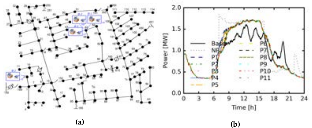
Fig. 5. The circuit diagram for (a) the modified IEEE 123-bus test system. The original circuit has a peak load of 3.6MW, 1.3MVAR and is to be representative of a very large residential subdivision in the U.S. Distribution system total active power for the (b) baseline and control cases. This is an aggregation of all building loads minus the power losses across the distribution system without considering any contributions from PV generation.
