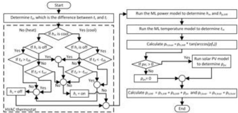
Fig. 4. Flowchart for the HVAC and building simulator that employs ML HVAC models as well as the PV simulator.
