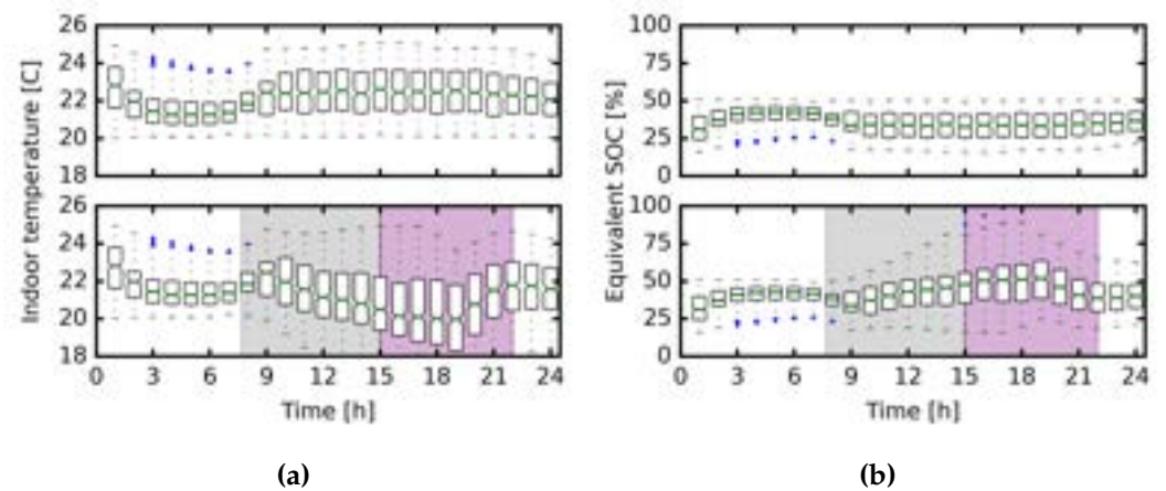
Fig. 13. Hourly average (a) indoor temperatures and (b) equivalent SOC, which is inversely related to indoor temperature, of all buildings for the baseline and P6 cases.
