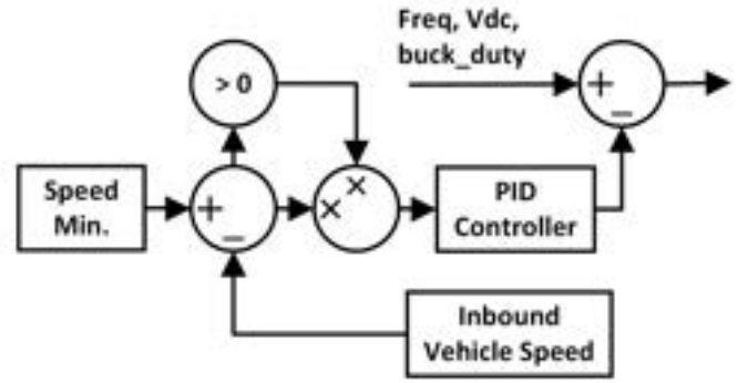
Fig. 3. Proposed control scheme to adjust power electronics parameters from the systems level, altering the real power output wirelessly transferred to the moving vehicle.
