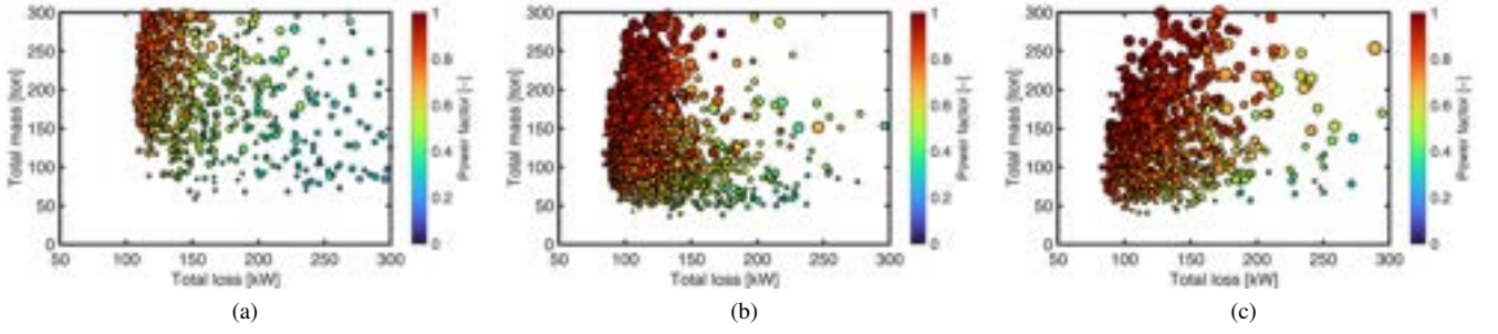
Fig. 4. Results of the multi-objective optimization showing the design distribution considering the total mass, total loss, power factor, and torque ripple for the generators using, (a) B_r = 0.4 T, (b) B_r = 1 T, and (c) B_r = 1.3 T. The size of the circle marker for each design is proportional to the torque ripple.
