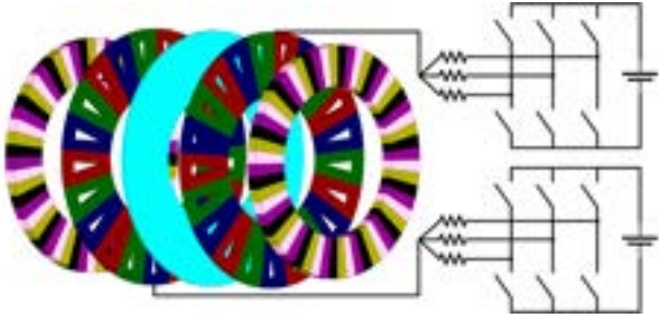
Fig. 6. Example CAFPM stage implementation with two independent, coreless stator modules, each with a PE converter.
