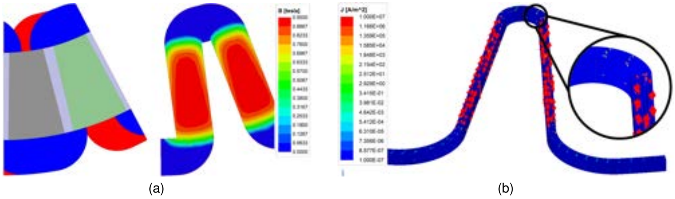
Fig. 2. Wave winding stator single pole pair 3D FE model and flux density distribution (a) and a diagram of the eddy current path in one turn (b). Since the dual rotor's magnets do not cover the coil's end windings, eddy current path is limited to the radial portion, shown in the detailed view.
