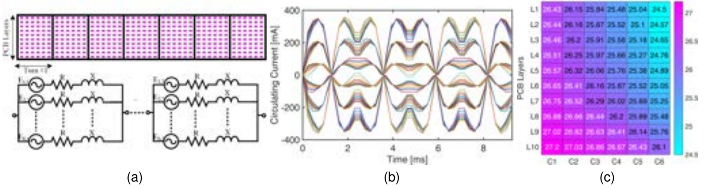
Fig. 5. Wave winding PCB stator diagrams including the conductor cross section for one phase and equivalent circuit for one layer (a), the open-circuit circulating currents in parallel traces within one turn (b), and a heat-map of the calculated induced voltages between copper traces within one turn over ten layers (c).
