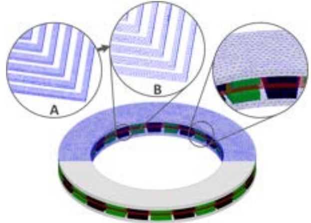
Fig. 9. The 3D FEA model for loss analysis that shows the employed tetrahedral mesh elements with zoomed-in views in different versions.
