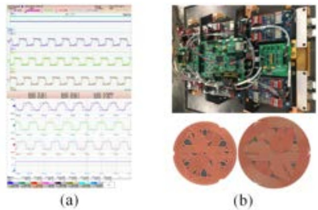
Fig. 3. The proposed shielding design is for an existing set of rotating-field 3-phase coils with examples shown here with voltage and current waveforms from a previous experimental benchmark (a) and example power electronics and coil geometry of the prototype which currently employs conventional ferrite shielding (b) [2].
