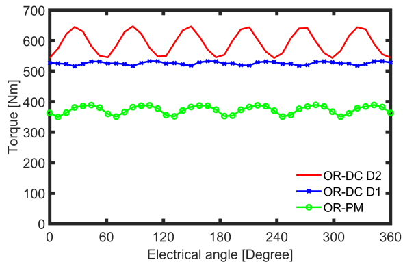
Fig. 6. Torque waveform for OR-PM, OR-DC D1, and OR-DC D2 designs.
