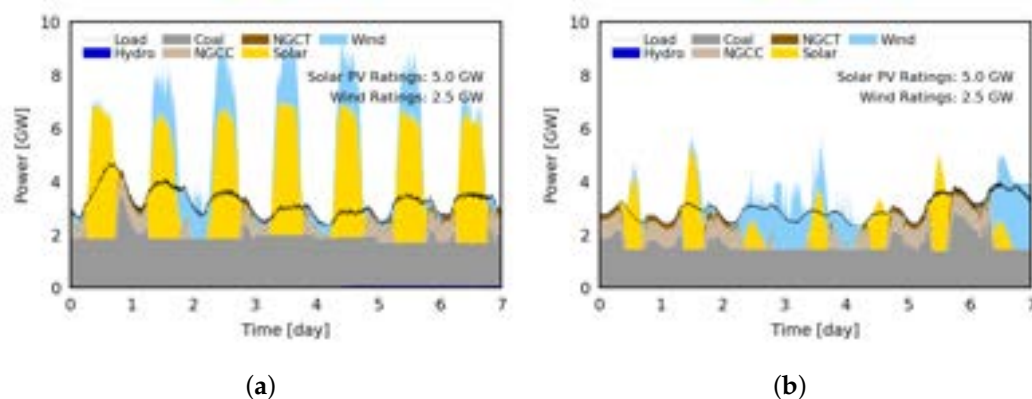
Figure 6. Example weeks of economic dispatch with a coal-dominated scenario for (a) a high renewable capacity factor week from May 8–14 and (b) low renewable capacity factor week from January 8–14. Renewable output may need to be significantly curtailed compared to natural-gas dominant generation due to slow turn-down and start-up times specific to coal operation as a base load.
