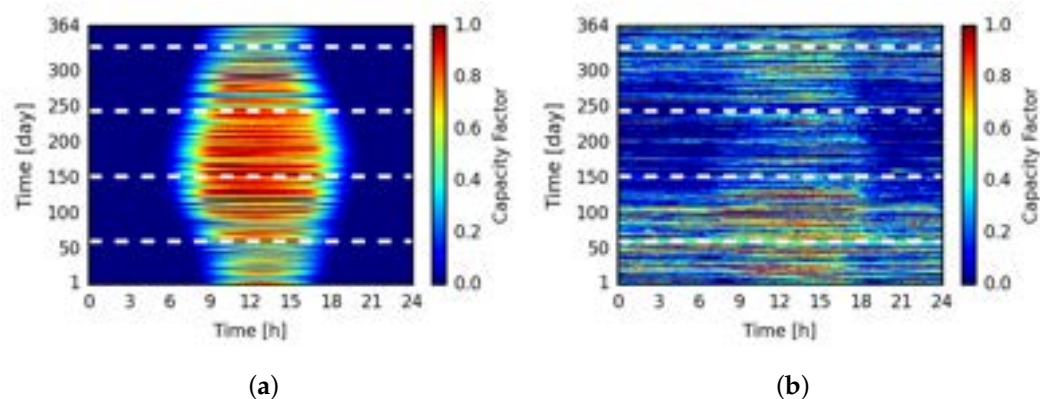
Figure 2. Kentucky state-wide utility solar PV (a) and land-based wind (b) aggregated minutely generation capacity factor across the year with white dotted lines differentiating meteorological seasons. Resources were found to be beneficially disjoint and complementary with high output from solar PV in the summer months and wind in the winter months.
