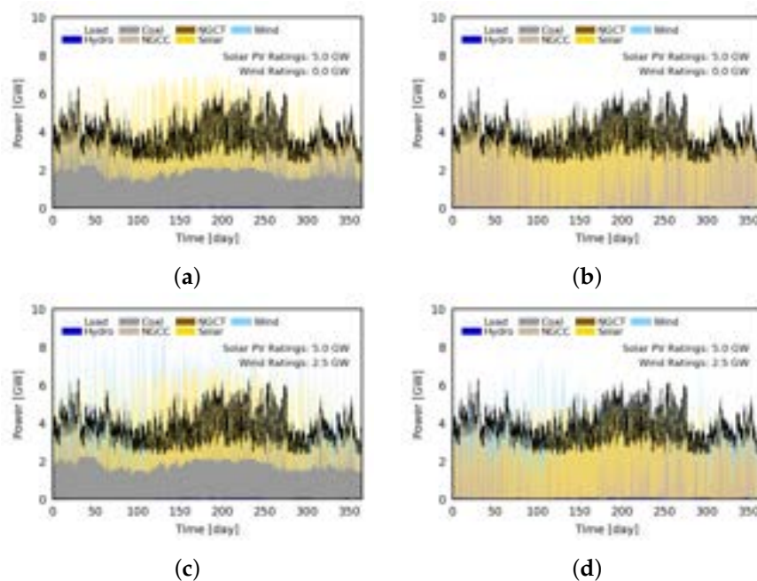
Figure 5. Full year minutely simulation of optimal power dispatch for 4 decarbonization scenarios: (a) C_S ; (b) NG_S ; (c) C_{SW} ; and (d) NG_{SW} . Compared to natural gas at the same solar PV ratings, coal-dominant cases suffer from a significant under-utilization of available VRE generation.
