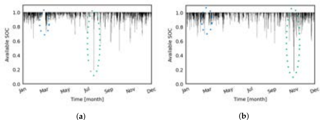
Figure 14. Battery energy storage sized to solve minutely imbalances with plotted available SOC across the year for natural gas dominant generation with (a) 20 GW of solar PV capacity, 10 GW of wind capacity, rated power of 4.6 GW, and energy capacity of 0.41 GWh; and (b) 6.5 GW solar, 3.25 GW wind, 2.5 GW power, and 0.112 GWh energy capacity. Dominant renewable generation significantly shifts the expected maximum peaking power to meet quick drops in VRE output and BESS energy capacity is non-linearly related to renewable capacity.
