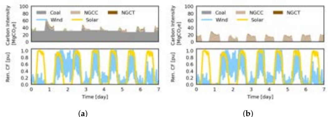
Figure 9. Example week of economic dispatch carbon intensity for a high renewable capacity factor weeks with (a) coal-dominant support and (b) natural gas-dominant support, respectively. Large spikes in carbon intensity occur in response to renewable power fluctuation. Quick spikes appear to peak and meet demand which can be compensated for with short term energy storage or demand response.
