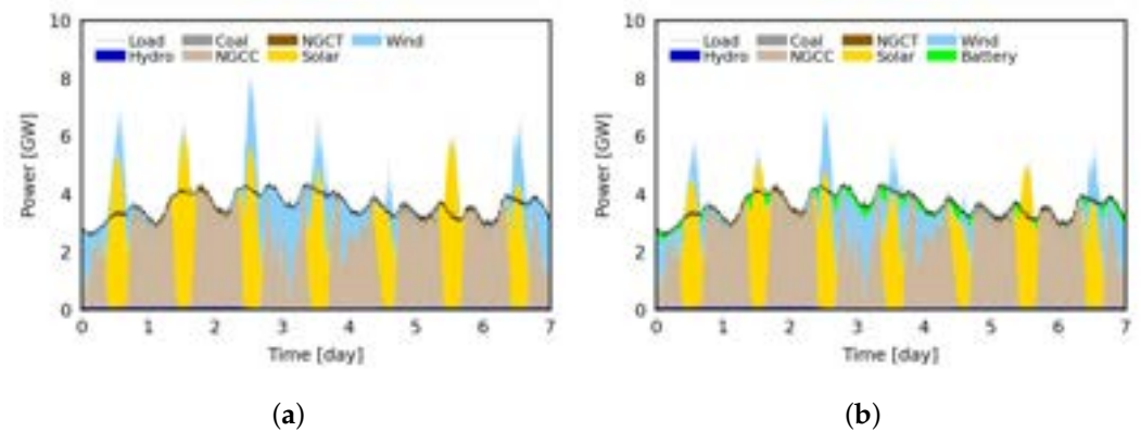
Figure 12. Example week of economic dispatch for in the critical month of January for a gas dominated system with for 6.5 GW solar PV and 3.25 GW wind capacity with (a) dispatch with pre-defined weather data and (b) reduction in VRE output by 15% post-dispatch and battery energy storage for matching load demand.
