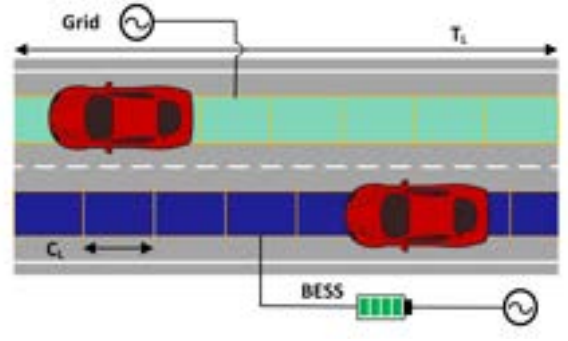
Fig. 6. Split-track hybrid DWCS configuration with a grid-connected BESS charging during off-hours and discharging to power one track of the roadway during peak periods to shift peak power consumption.
