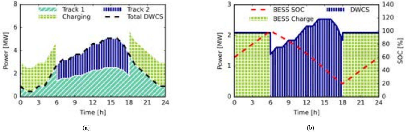
Fig. 7. Power profile for a hybrid DWCS configuration in (a) a stacked two track hybrid DWCS arrangement with traffic redirected towards both tracks for charging during peak loading periods between 6:00 and 18:00 and (b) the input/output power into the second track within the same time period with an integrated BESS system alongside the dynamic BESS SOC.
