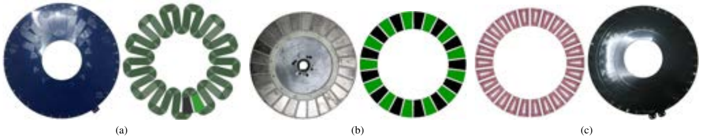
Fig. 1. PCB stator simulation models and motor hardware components for the wave winding stator (a), dual 26 pole rotor (b), and the spiral winding stator (c) used for ANSYS Maxwell simulation and the experimental motor prototype.
