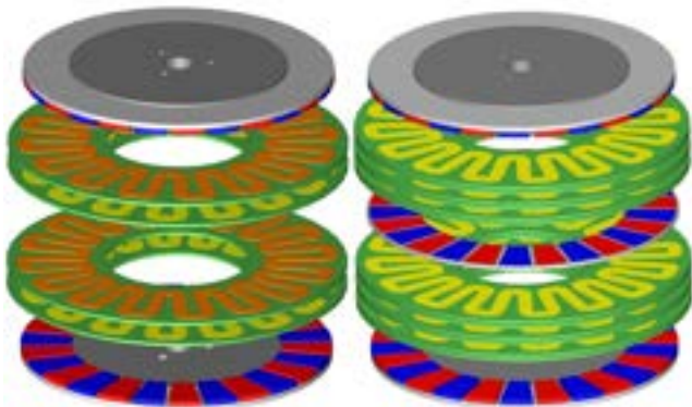
Fig. 2. For coreless machines, multiple stacks of stators and rotors can be employed in a modular approach to achieve a specified power rating.
