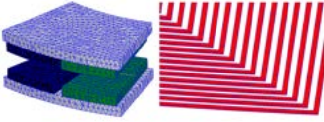
Fig. 5. Meshing of detailed trace-by-trace model of the proposed PCB spiral winding coreless AFPM machine. The rotor back iron and magnets are shown on the left and the PCB traces are shown on the right.
