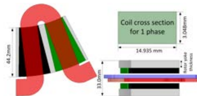
Fig. 6. A single coil of the selected coreless AFPM PCB design. This section represents 1/13th of the full 2 phase design model and the full model's results can be extrapolated through geometry.
