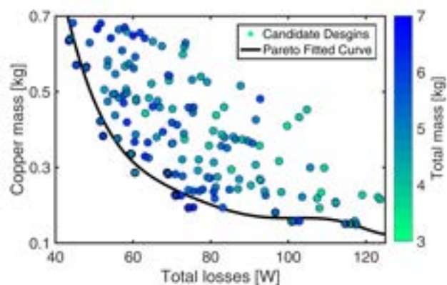
Fig. 4. The Pareto front and all the other designs evaluated by 3D FEA throughout the differential evolution for the 2-phase PCB stator AFPM with wave winding.
