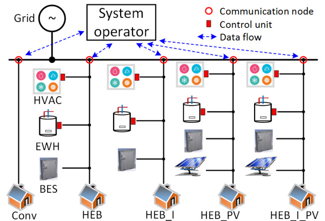
FIGURE 2. The proposed system model includes five types of SET homes, each type being representative of thousands of individual houses. In the study, the load data for the business and industrial sectors is provided by experimental measurements.
