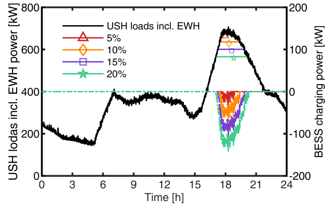
FIGURE 16. The aggregated total USH loads with peak reduction achieved by BESS. Only the discharge operation of BESS are shown.
