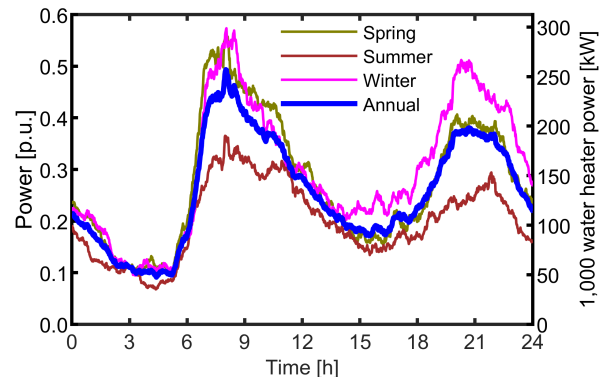
Fig. 7: The generic power curve created based on the BPA data for Spring, Summer, and Winter for the year of 2018. The annual curve, which includes the data from the three seasons, is used to generate the generic HPWH curve.
