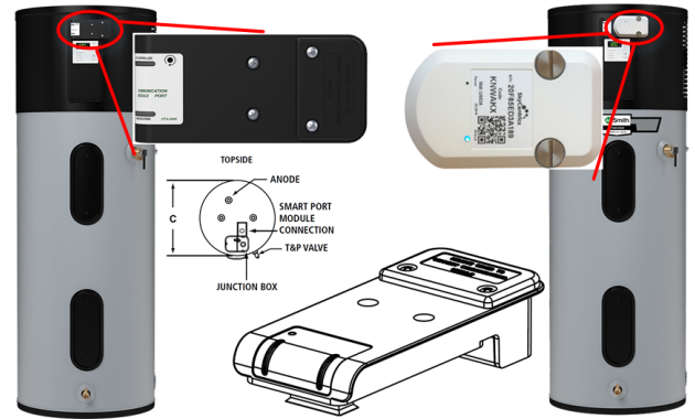
Fig. 1: The illustrative parts of A.O.Smith “Energy Smart” model and CTA-2045 standard port. The “Energy Smart” controller is smart grid ready and implements standardized communications for demand response.
