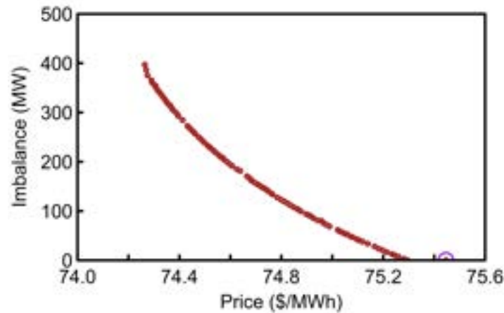
Figure 5. The multi-objective optimization Pareto front for example minute. The selected design is the one with the minimum imbalance for every case.
