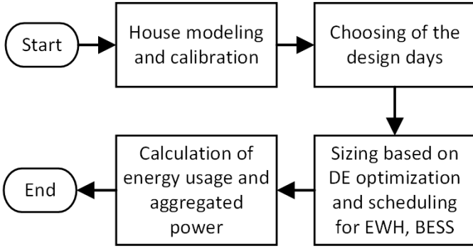
Figure 7. Procedure for the sizing of HyPVES, calculation for electricity spending of NZE home and aggregated power of the distribution system.
