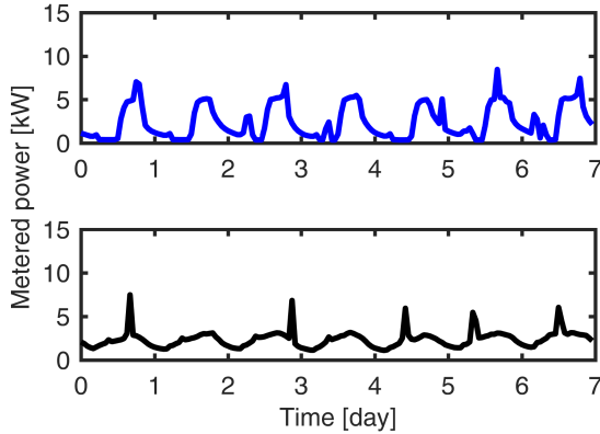
Figure 3. Results from two building simulation tools on the daily and weekly load for a typical 3-bedroom, 1.5 bathroom house calculated during a summer week in California with CBECC-Res 2019 (top) and EnergyPlus(bottom).
