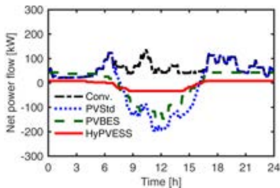
Figure 13. Power flow profile at node 634 of the IEEE 13-bus test system from Fig. 11 on a winter day.
