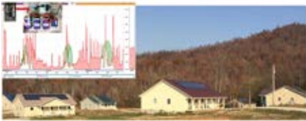
Figure 2. A newly developed field demonstrator with twelve near-NZE houses in southern Kentucky, which are modeled within the INSPIRE+D co-simulation framework and validated with measured load data.
