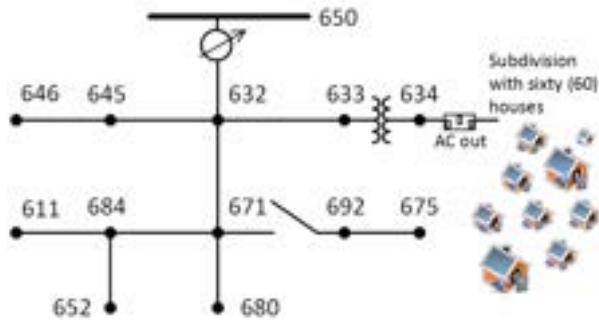
Figure 11. The IEEE 3-phase single line diagram 13-node feeder test case is adopted for the district level simulation. Sixty NZE houses are linked to node 634.
