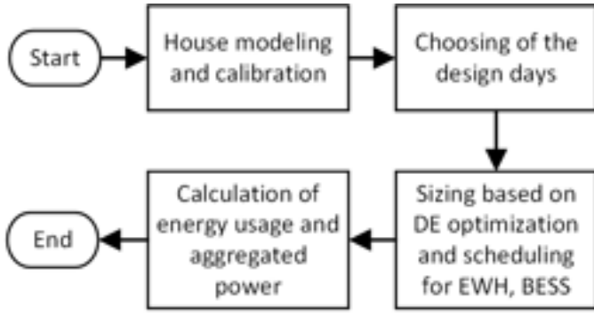
Figure 7. Procedure for the sizing of HyPVESs, calculation for electricity spending of NZE home and aggregated power of the distribution system.
