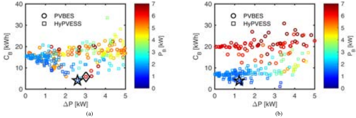
Figure 9. The DE results of battery sizing for southern Kentucky on a representative (a) summer's day and (b) winter's day. A battery rated for 4.1kWh/1.3kW is chosen based on the summer case and marked with a \star . The sized battery has a maximum output power fluctuation of 2.6kW and 1.2kW for the summer and winter days, respectively. Though better choices are available on the winter day, the limitation is set by the summer.
