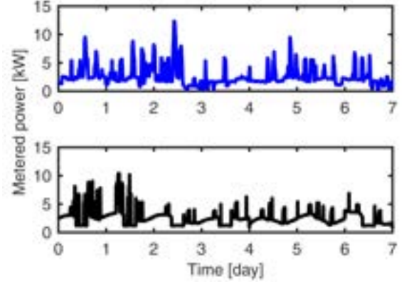
Figure 4. Experimental (top) and EnergyPlus simulation data for a house in southern KY in a winter week. The total weekly energy usage comply satisfactorily.
