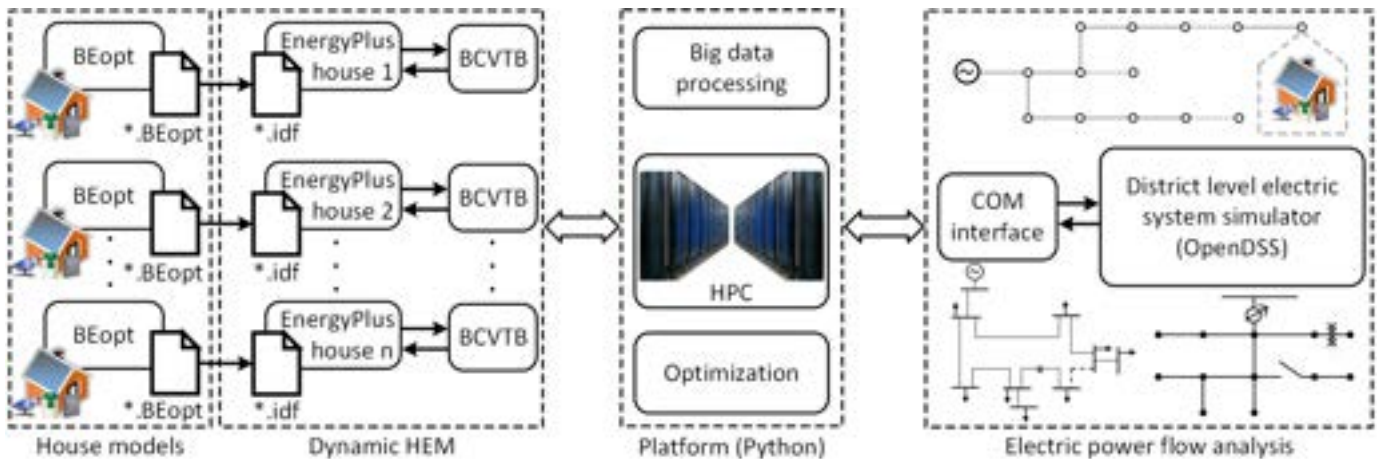
Figure 1. The INSPIRE+D co-simulation framework, including four parts. Thousands of single house energy models can be simulated in parallel through a high performance computing (HPC) system.
