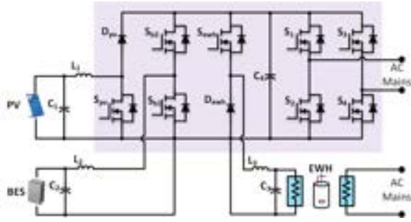
Figure 5. Example power electronic interface for an NZE house. The battery storage, electric water heater and PV array are interconnected with the DC bus via a multi-port converter.
