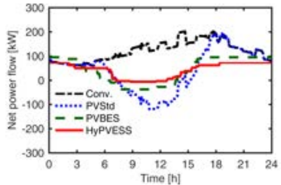
Figure 12. Power flow profile at node 634 of the IEEE 13-bus test system from Fig. 11 on a summer day.
