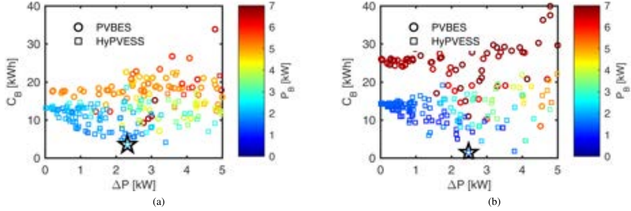
Figure 8. The variation of battery energy capacity, C_B with grid power fluctuation, \Delta P evaluated for several thousand values of P_1 , P_2 and t_1 in NZE homes equipped with only BESS and PV (PVBES), and the hybrid PV energy storage system (HyPVES) on a representative (a) summer's day and (b) winter's day for California.
