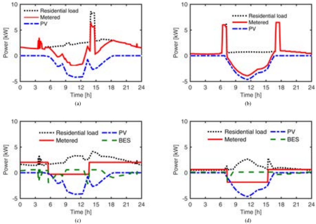
Figure 10. Power flow in a home equipped with a solar panel, but no storage, on (a) a summer's day, and (b) a winter's day. Power flow in a home with solar panels and coordinated control of energy storage systems on the same (c) summer's day and, (d) winter's day.
