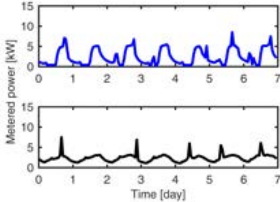
Figure 3. Results from two building simulation tools on the daily and weekly load for a typical 3-bedroom, 1.5 bathroom house calculated during a summer week in California with CBECC-Res 2019 (top) and EnergyPlus(bottom).
