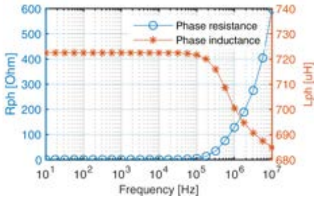
Fig. 6. Phase resistance and inductance vs. frequency from FEA. Eddy currents in conductors are modeled whereas the coreloss effect on the field is not considered.
