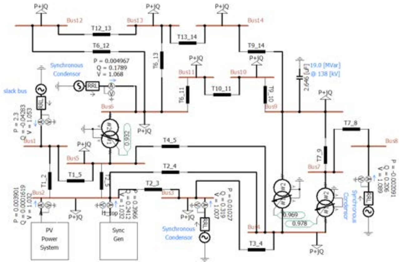
Fig. 11. Modified IEEE 14 bus system with the PV system incorporating a BESS supplying part of the power at Bus no. 2
