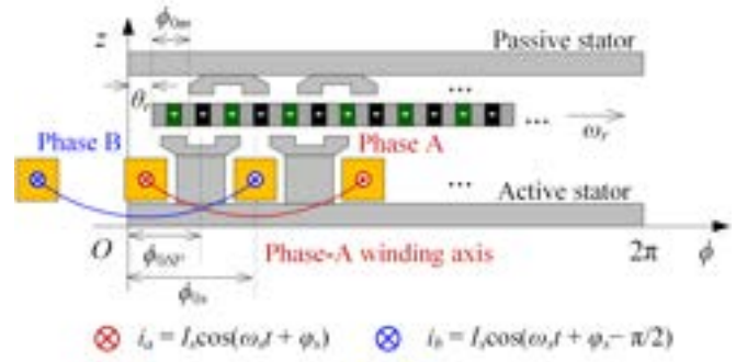
Figure 3. The coordinate system used for theoretical analysis. The proposed VTFM machine with 1-active and 1-passive stator is modeled. It may be noted that the phase sequence is opposite to the rotating direction of the spoke rotor, which is different from conventional PM machines.
