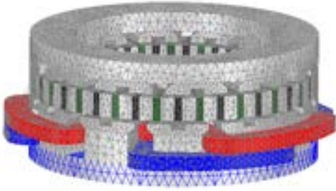
Figure 5. Mesh plot used in the 3D FEA model for the VTSM example machine with 16 stator slots and 56 rotor poles. The full problem featured 239193 tetrahedral elements and a quarter model is analyzed to reduce the computational burden.
