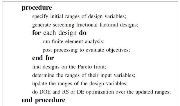
Figure 3. Procedure for the proposed DOE-algorithm. Initial studies are conducted over a wide search space, designs on the Pareto front identified, and the ranges of independent variables updated.
